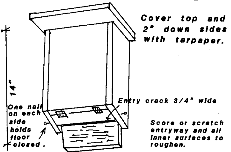
FRONT VIEW as mounted on building
